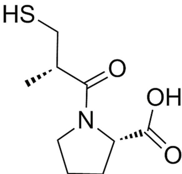
Figure 3: captopril's chemical structure.
